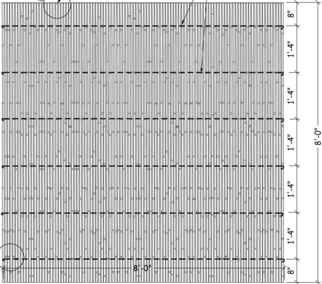
GALVANIZED WIRE THROUGH PRE-DRILLED HOLES IN BAMBOO, SECURED AT ENDS OF FENCE SECTION.
